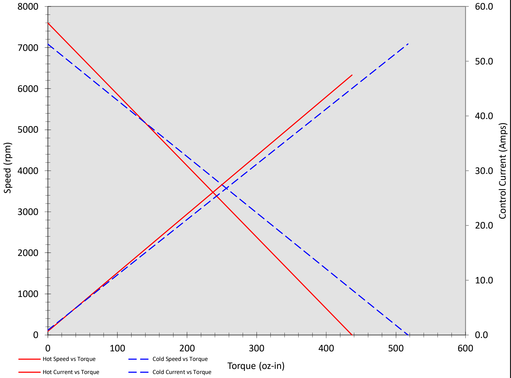
Performance: Type 34B4BEBL - 0.40 HP at 48 Volts
