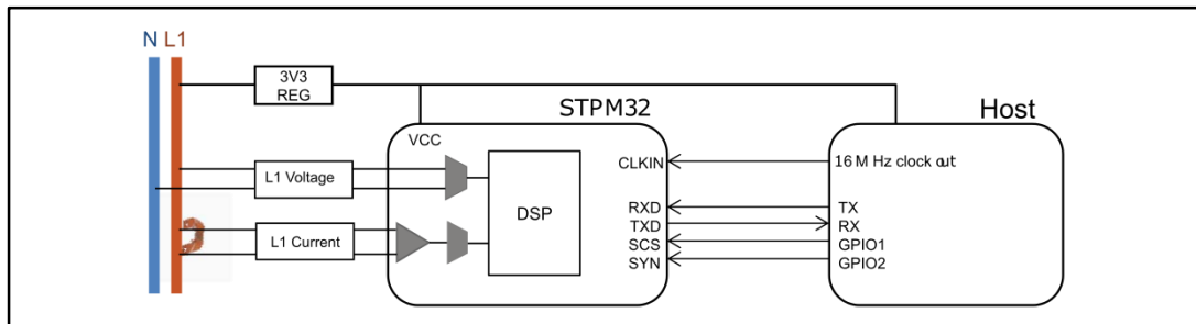
Figure 1: Connection through UART peripheral
