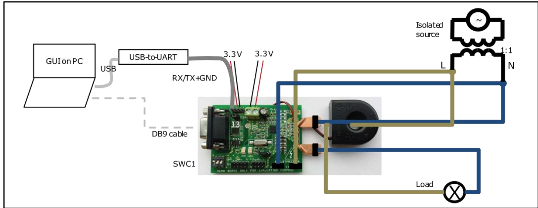
Figure 15: Connection to UART interface
