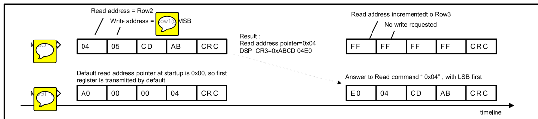
Figure 9: Frame sent and received from the device
