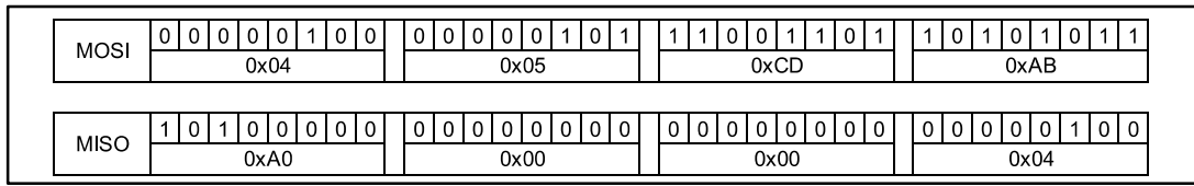
Figure 10: SPI bit flow
