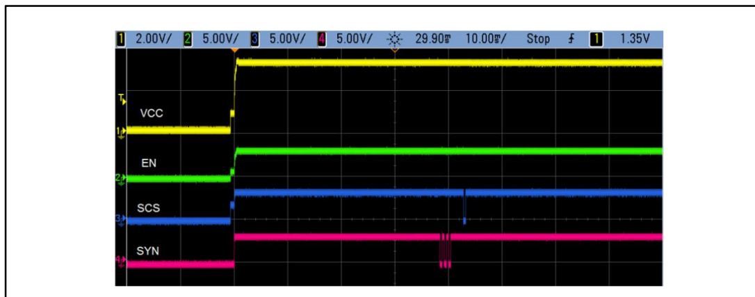
Figure 2: Timing example
