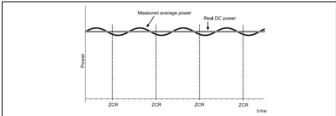
Figure 16: Power waveform
